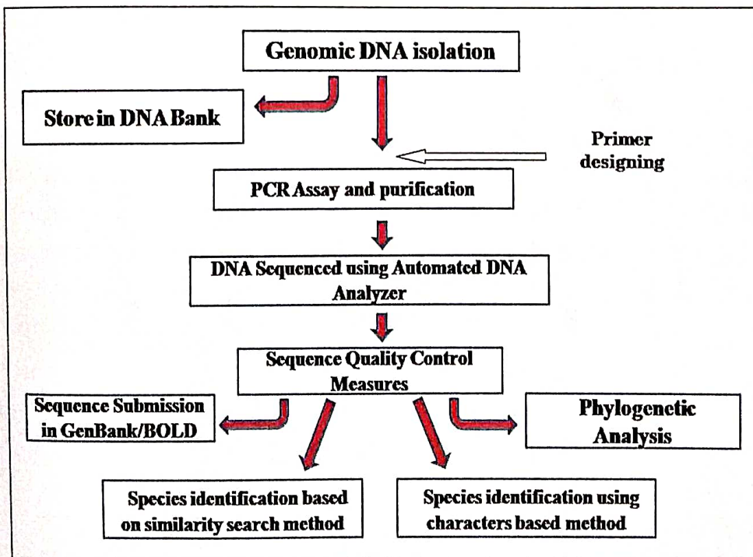
Fig. 1.1: Flow chart of DNA Barcoding
