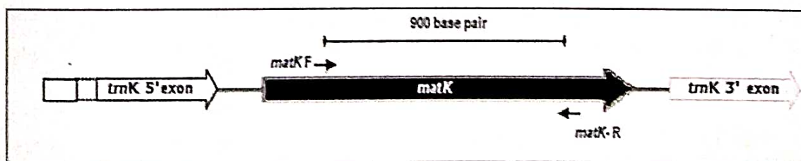
Fig. 1.3: Schematic diagram of maturase K gene of Cp-DNA
